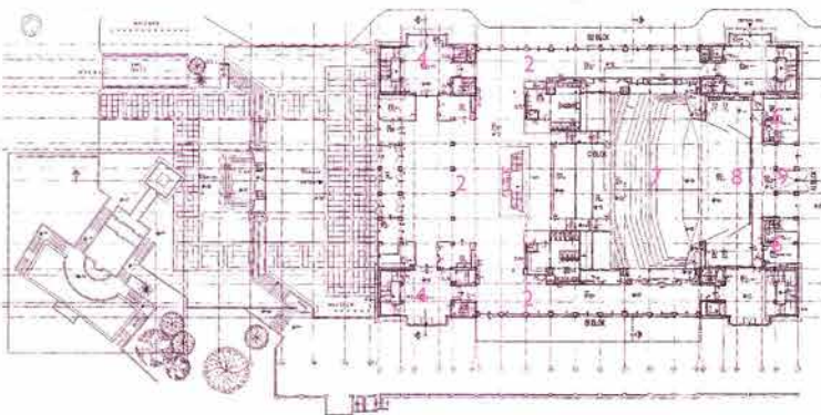
zemin kat planı / ground floor plan
