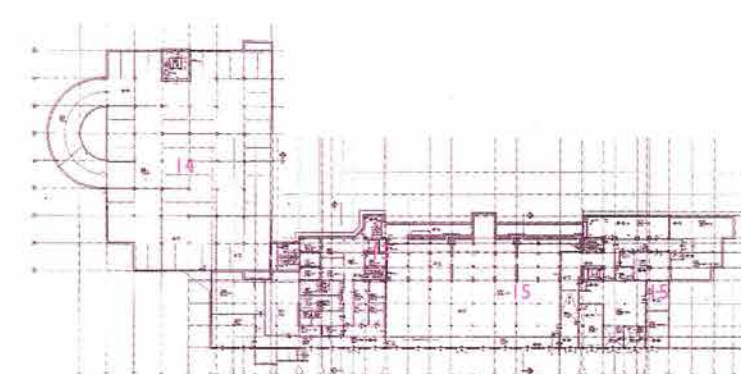
2. bodrum kat planı / 2. basement floor plan
